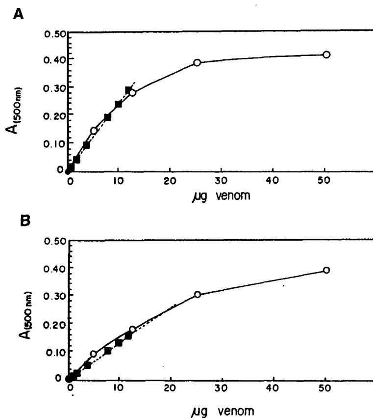
Fig. 2. B. cotiara venom LAO activity. * A=L-leucine substrate. B=L-phenylalanine substrate. (---○---○--- = assay range: 5-50 \mu g of venom). (-■-■- = assay range: 1-12 \mu g of venom). (*) 4-aminoantipyrine as chromogen.
